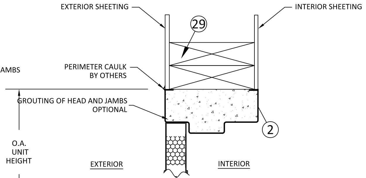
L 5 VERTICAL SECTION HEAD - 2X WOOD BUCK
