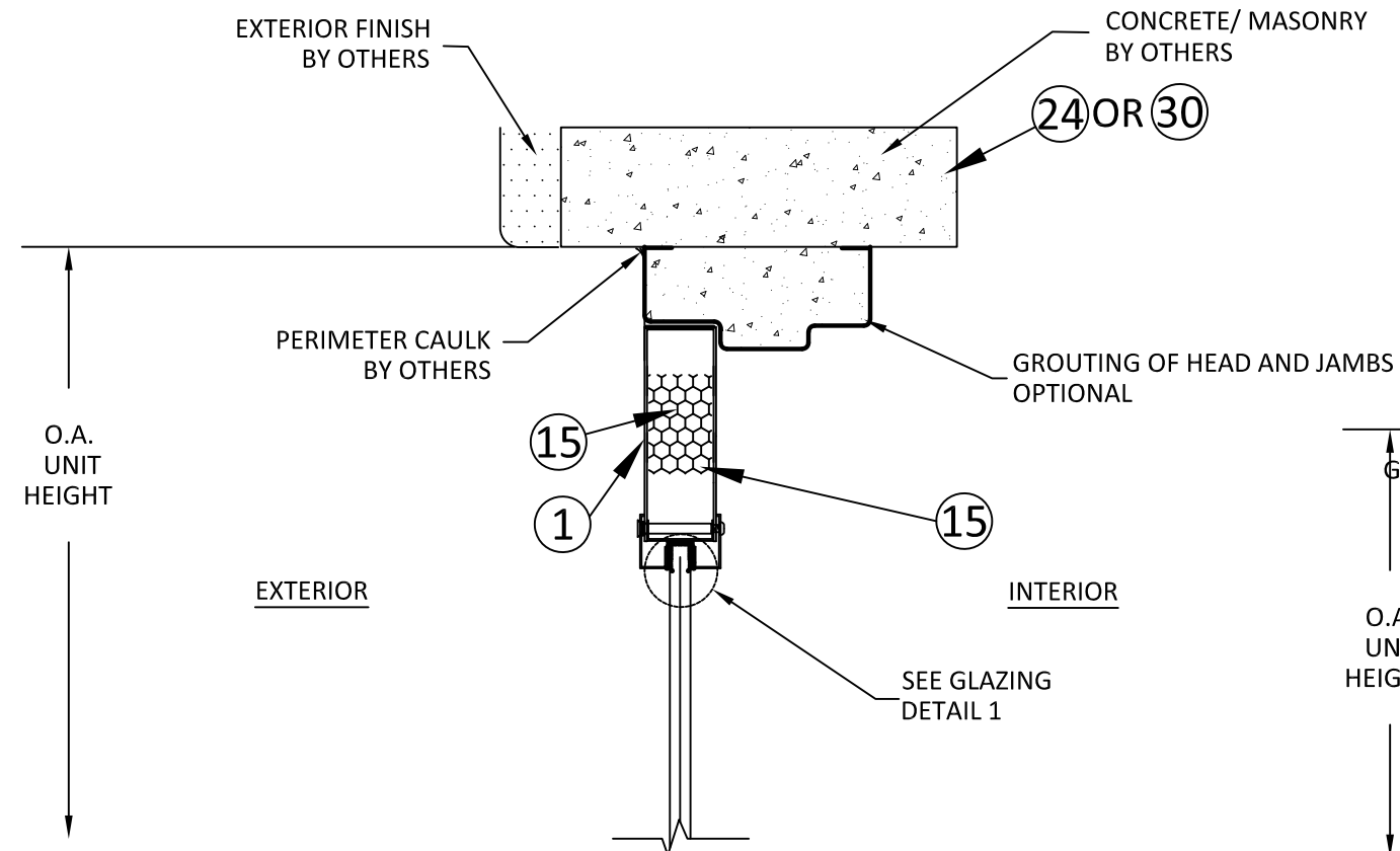
J 5 VERTICAL SECTION HEAD - CONCRETE
