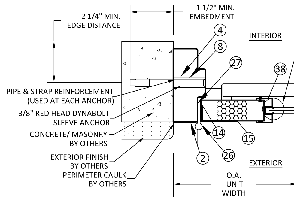
D HORIZONTAL SECTION 3 JAMB - CONCRETE SLEEVE ANCHOR
