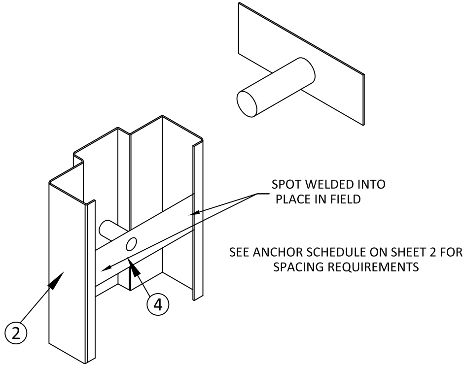
PIPE & STRAP ANCHOR
