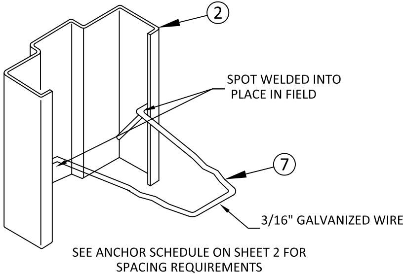
3/16" WIRE MASONRY ANCHOR
