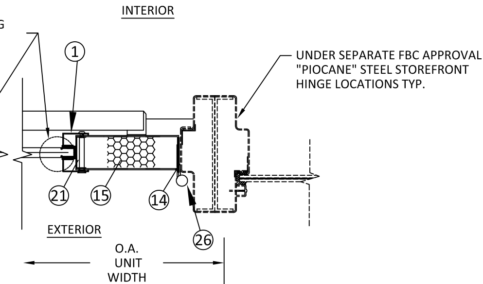
C HORIZONTAL SECTION 3 JAMB - GROUT FILLED CMU T-STRAP ANCHOR
